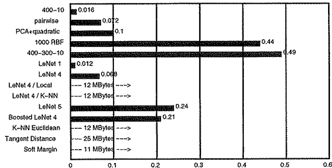
Figure 5: Memory requirements for classification of test patterns (in MBytes). Numbers are based on 4 bit/pixel for K-NN, 1 byte per pixel for Soft Margin, and Tangent Distance, 4 byte per pixel for the rest.
