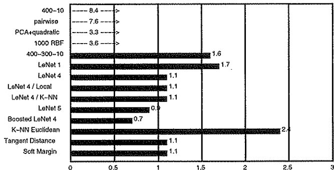
Figure 2: error rate on the test set (%). The uncertainty in the quoted error rates is about 0.1%.
